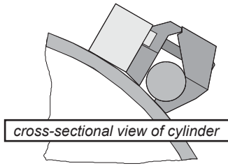
6" to 8" Bore NFPA Tie Rod
